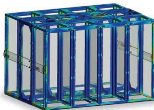
FEM calculations for the Arenit sifter frames.
